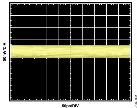
Figure 25. 3.25 Gbps Output Eye, 15 Meters CX4 Cable, PE = 0 (TP3 from Figure 24)
